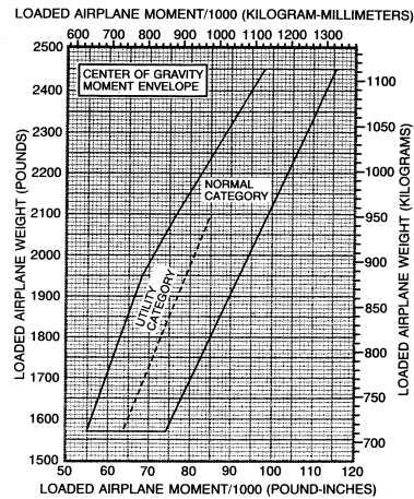
Figure 6-7. Center of Gravity Moment Envelope
