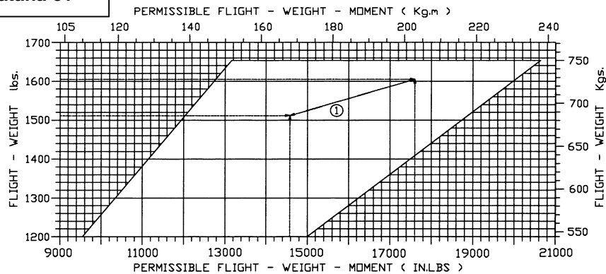
Figure 6-7. Center of Gravity Moment Envelope
